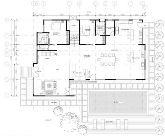
GROUND FLOOR PLAN 2710 SQFT
