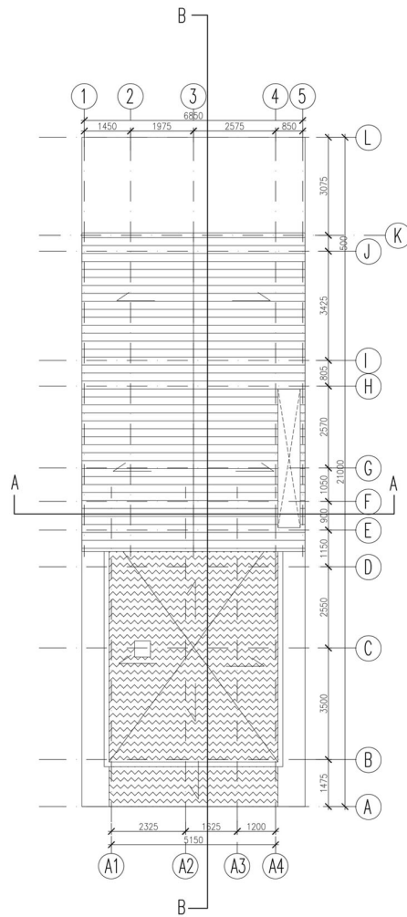
ROOF PLAN
