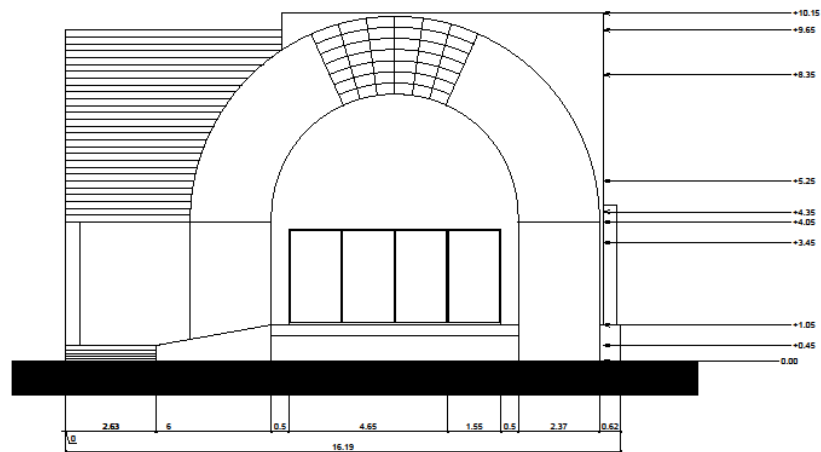
NORTHERN FACADE SCALE 1/100
