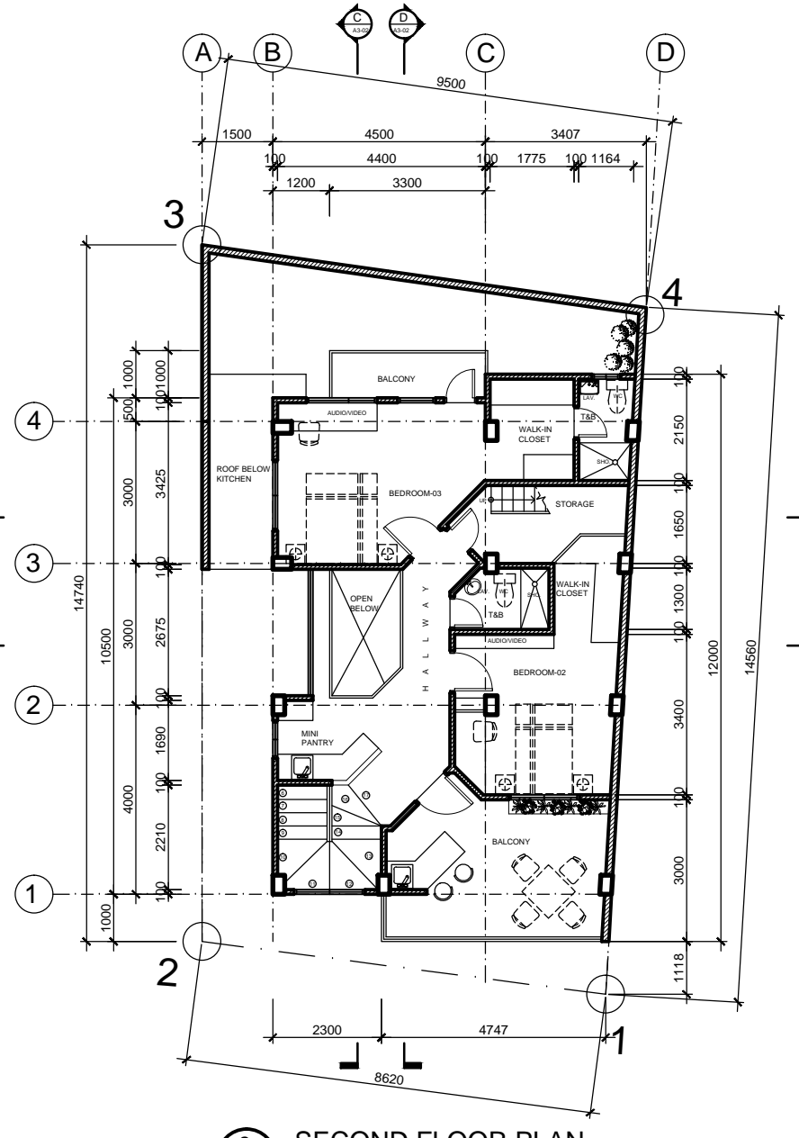
2 SECOND FLOOR PLAN A2-02 SCALE 1:100
