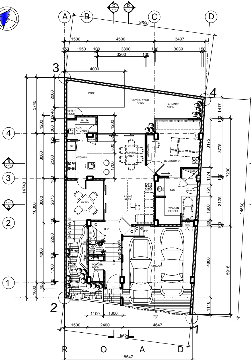
1 GROUND FLOOR PLAN A2-02 SCALE 1:100
