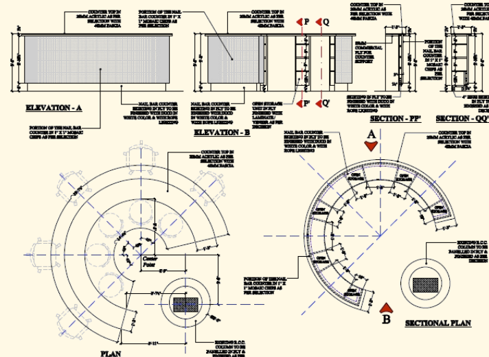
Wd : FURNITURE DETAIL - NAIL BAR
