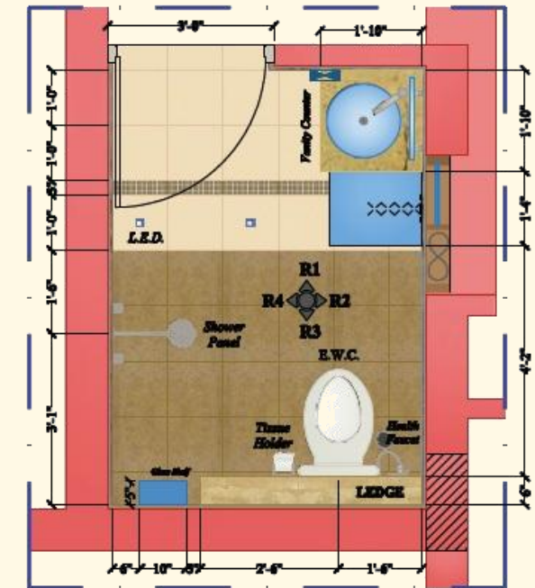
dd : FURNITURE LAYOUT
