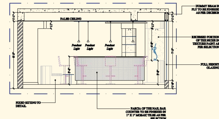
Wd : ELEVATION DETAIL - NAIL BAR
