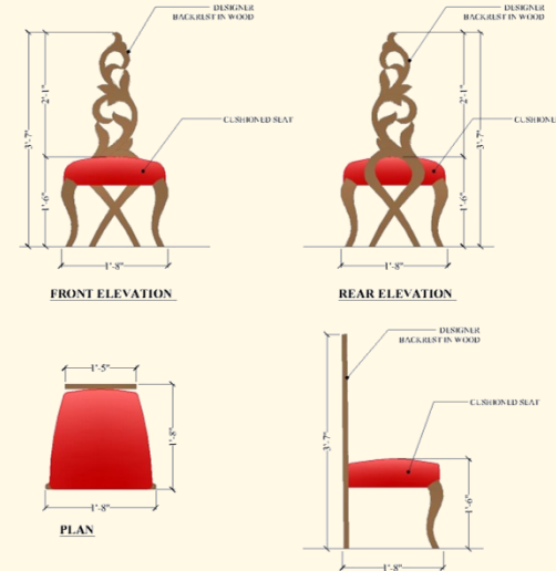
dd : CHAIR DESIGN – PRIVATE DINING
