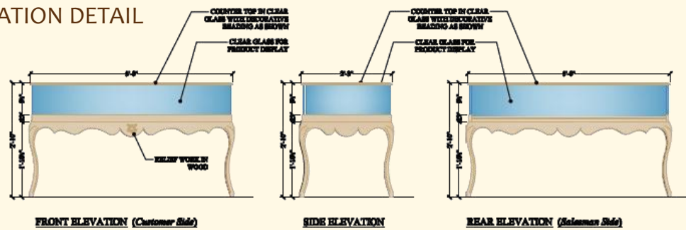
FRONT ELEVATION (Customer Side)
