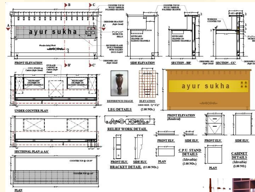
Wd : RECEPTION DESK
