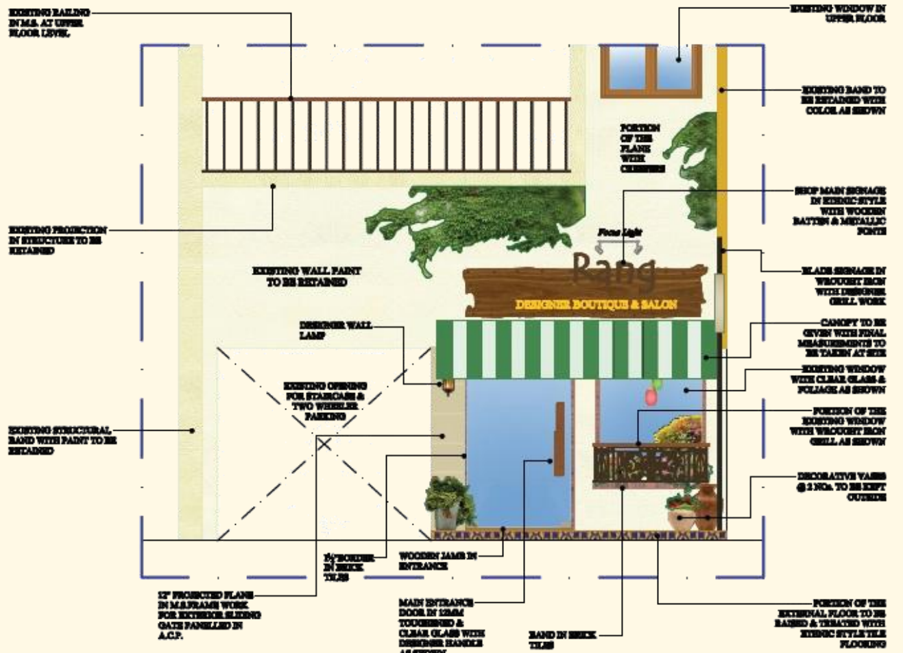
EXTERNAL ELEVATION DETAIL
