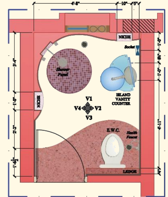
dd : FURNITURE LAYOUT
