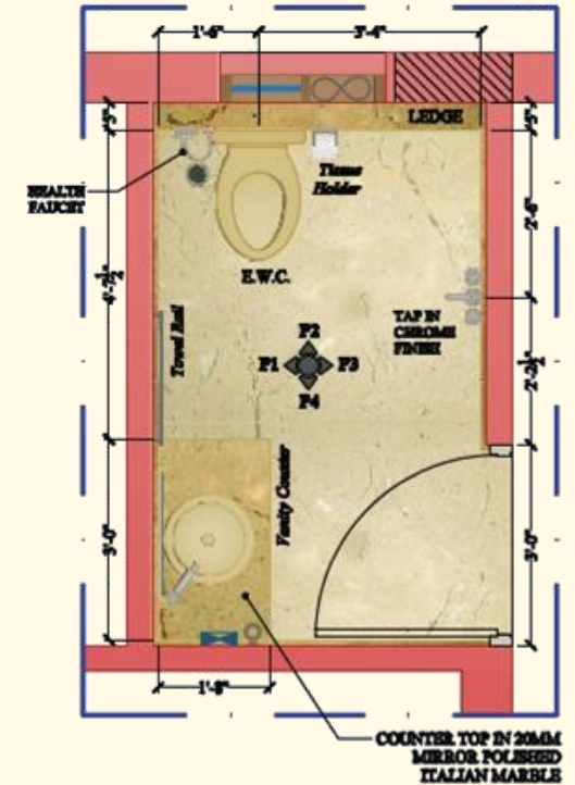
dd : FURNITURE LAYOUT
