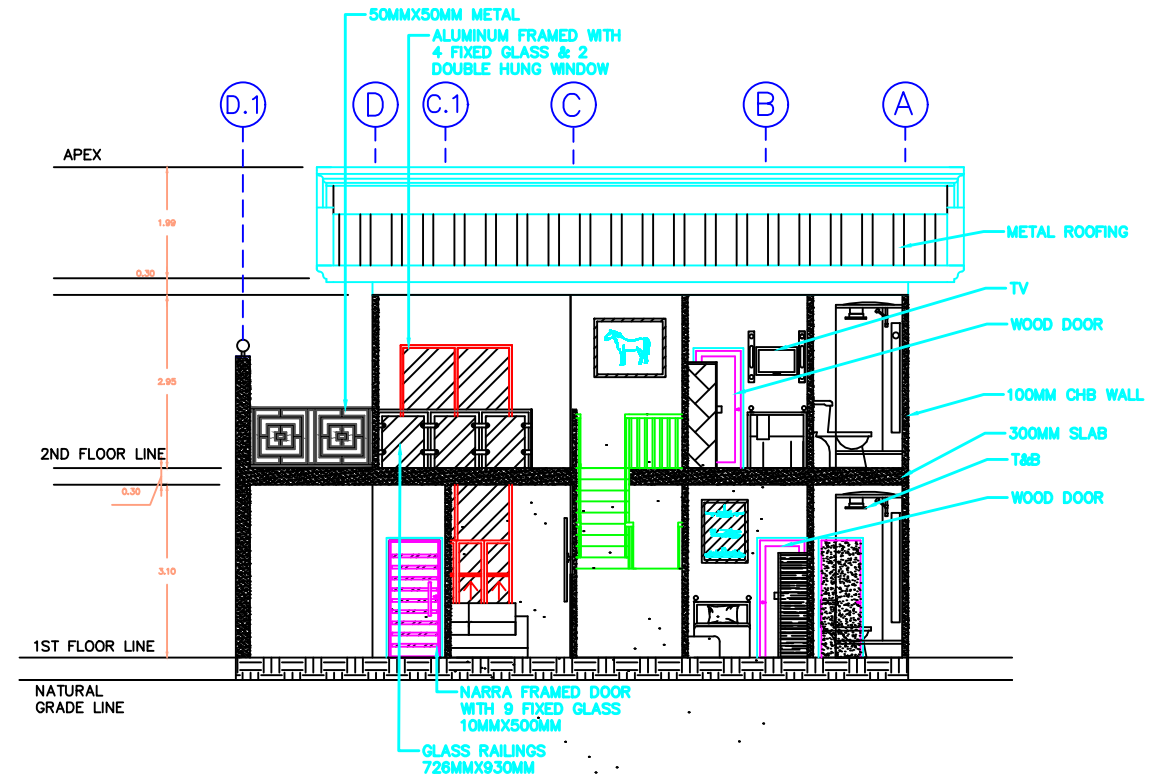
2-2 CUT SECTION SCALE NTS
