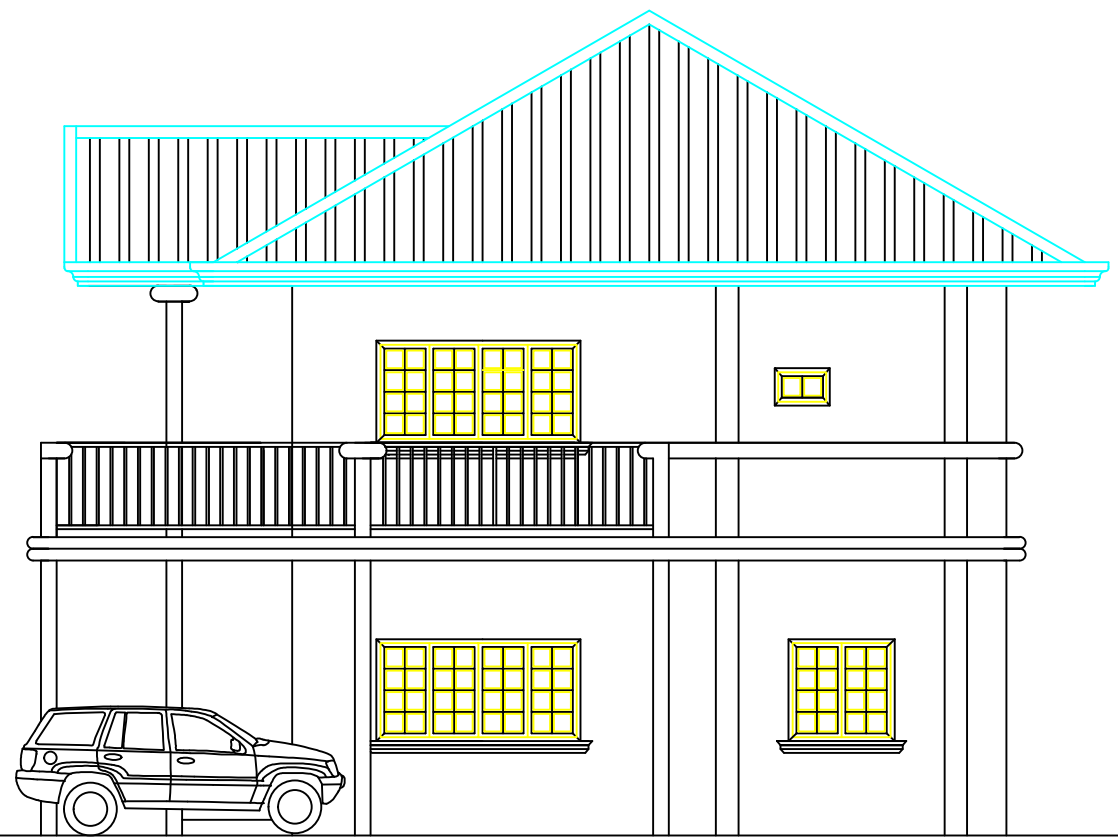
SIDE ELEVATION
