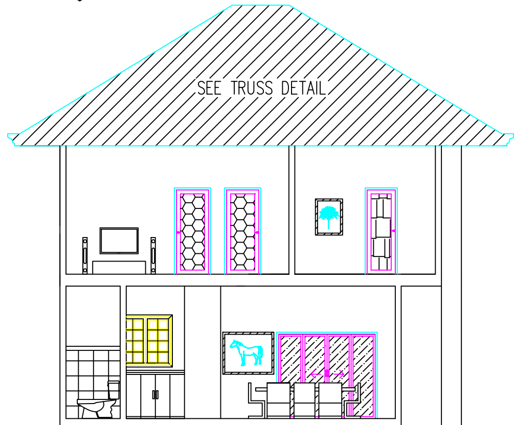
CROSS SECTION
