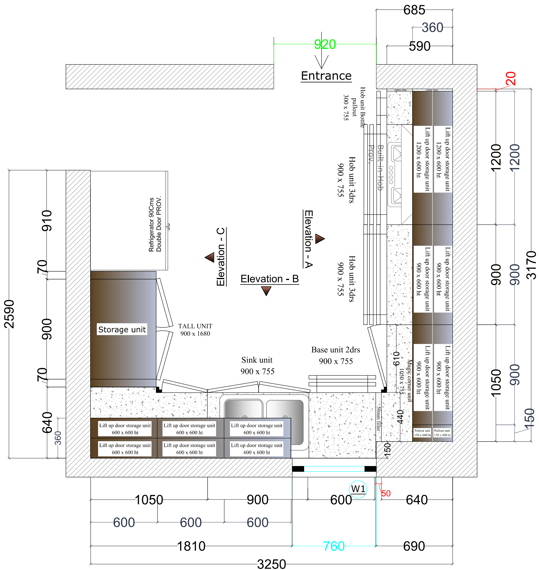
Wet Kitchen floor plan
