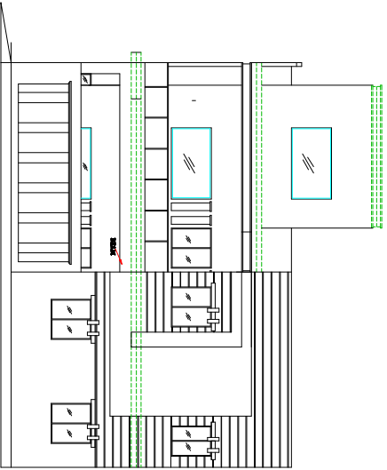
GROUND FLOOR SIDE ELEVATION WORKING
