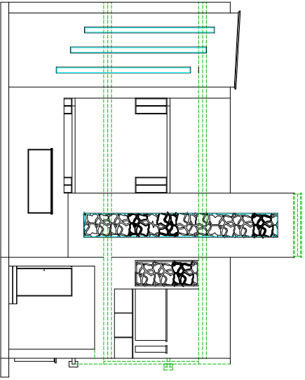
GROUND FLOOR FRONT ELEVATION
