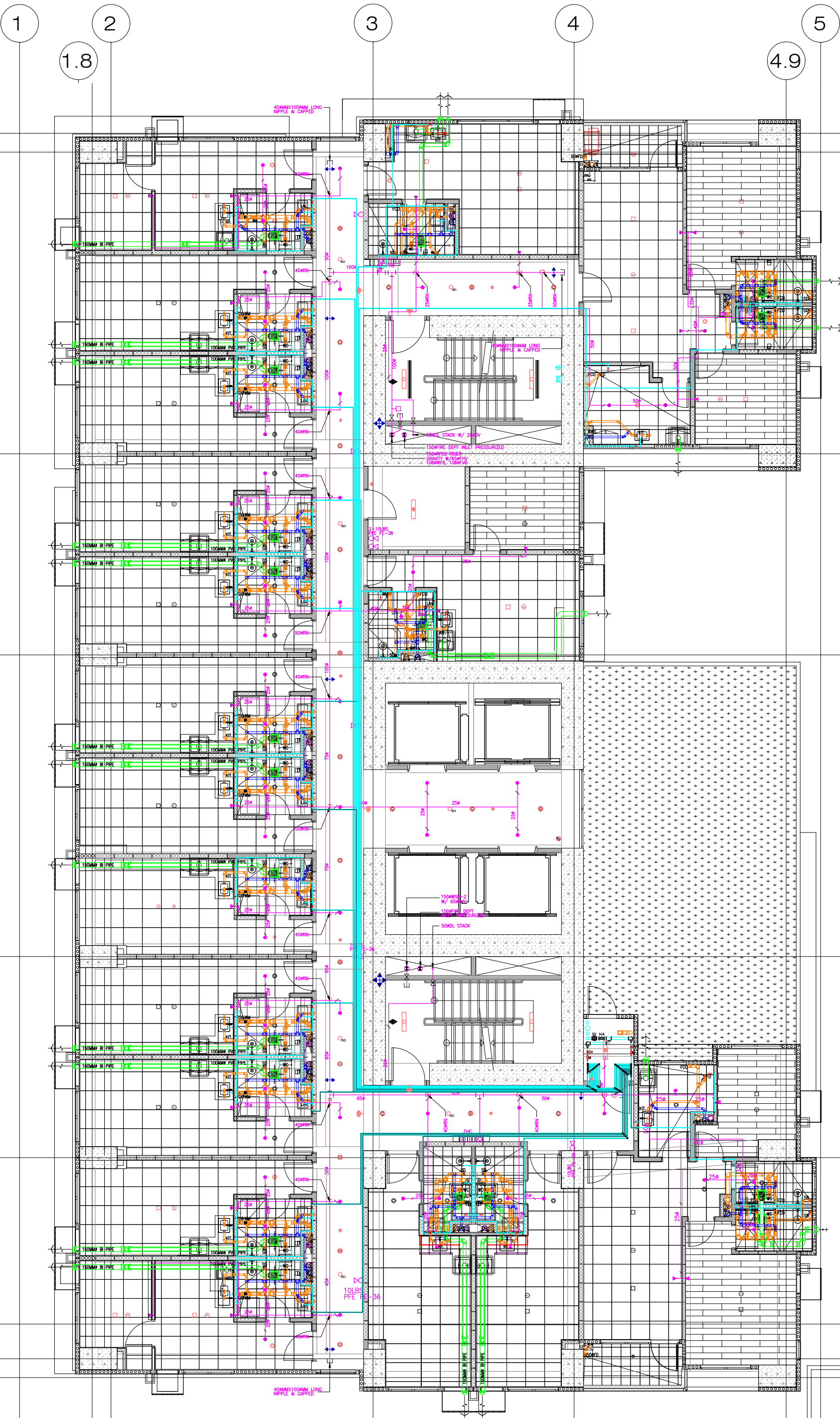
1 CSD RESIDENTIAL UNIT TOWER 1 TYPICAL 18TH TO 29TH FLOOR COMBINED SERVICES DRAWING SCALE 1:120M
