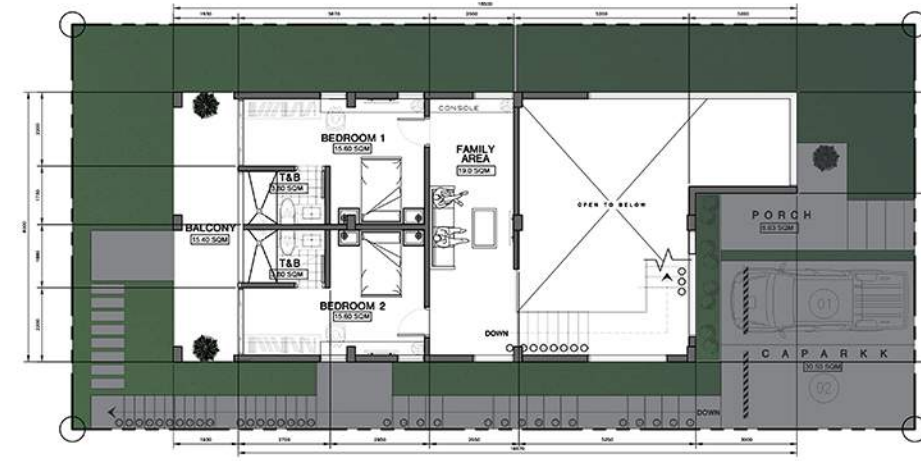
SECOND FLR.PLAN
