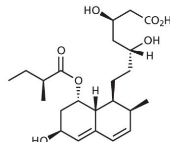
Pravastatin IC_{50}=1900 nM
