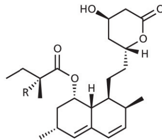
Lovastatin (R=H) IC_{50}=24 nM Simvastatin (R=Me) IC_{50}=11 nM
