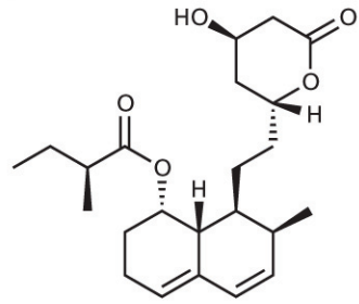
Compactin IC_{50}=23 nM (Mevastatin)
