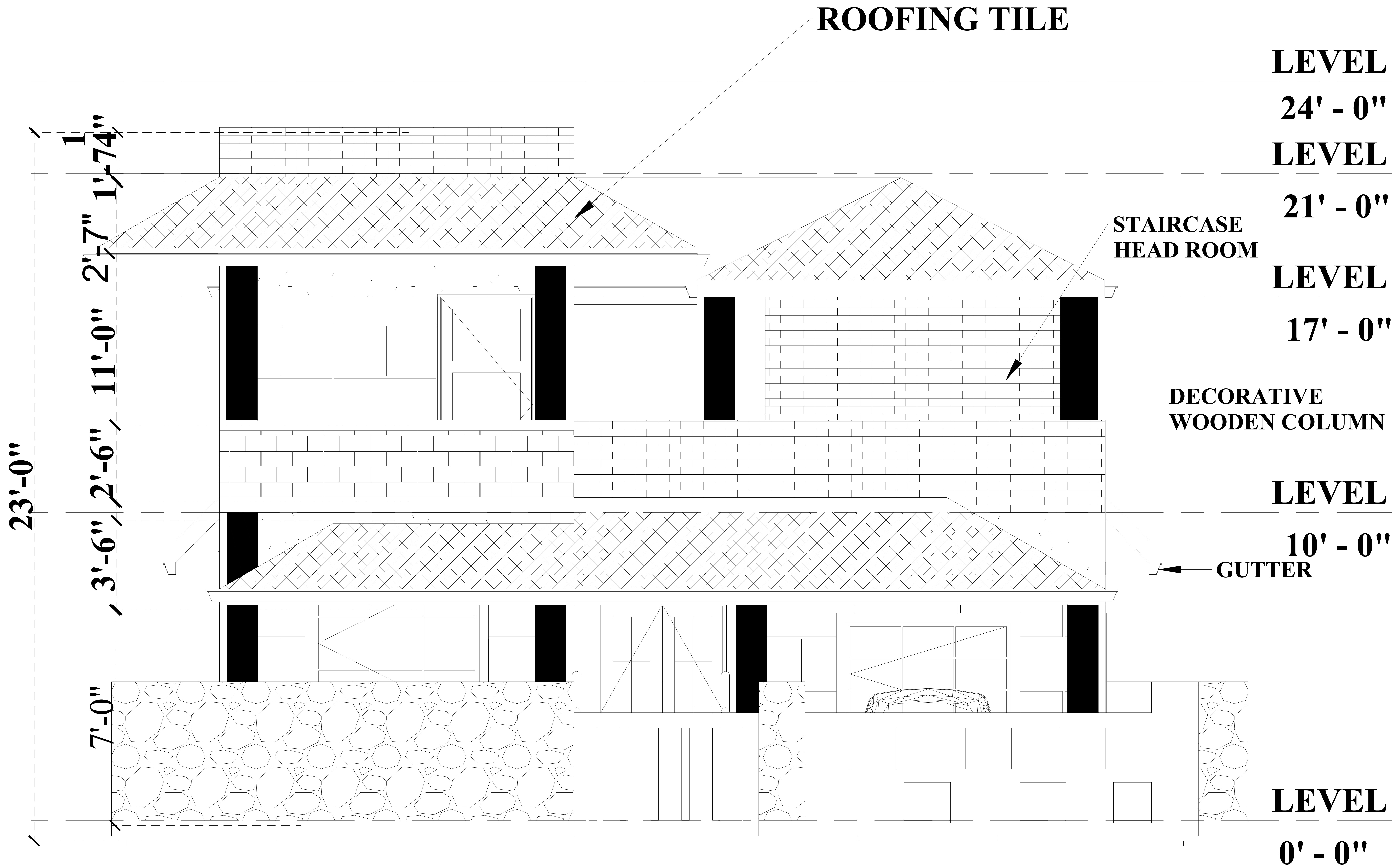
FRONT ELEVATION
