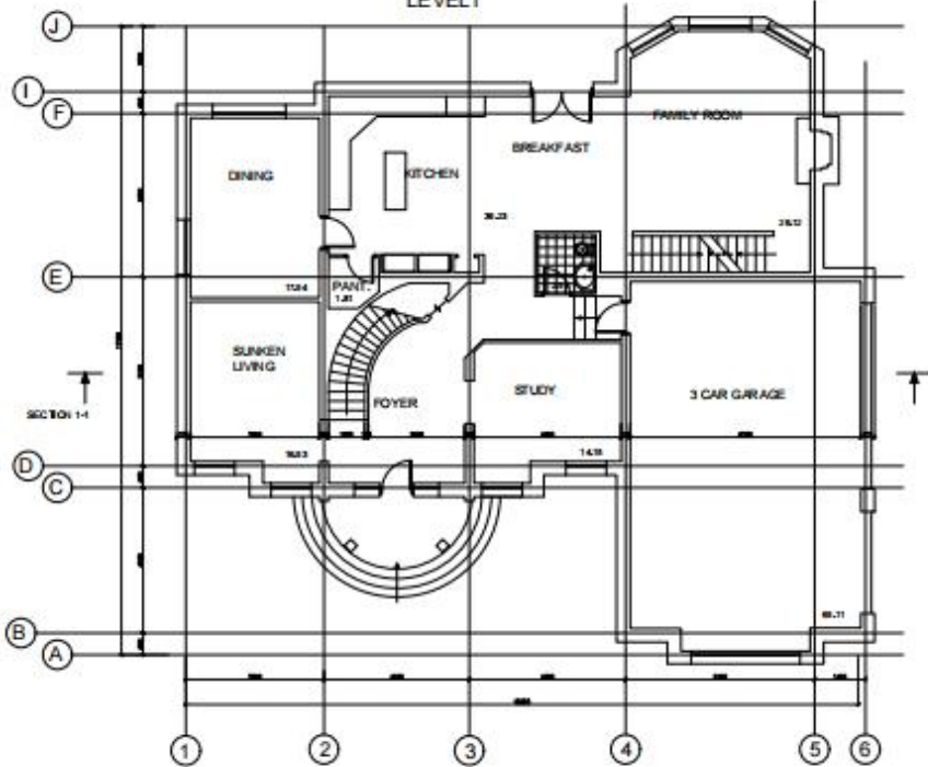
LEVEL 1
