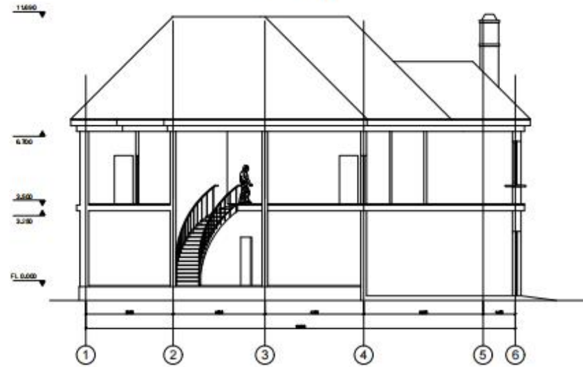
SECTION 1-1
