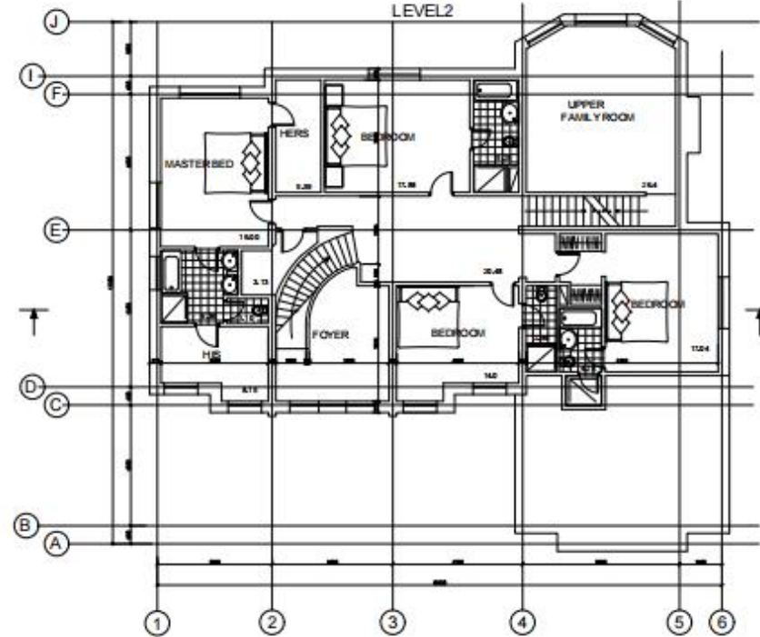
LEVEL 2
