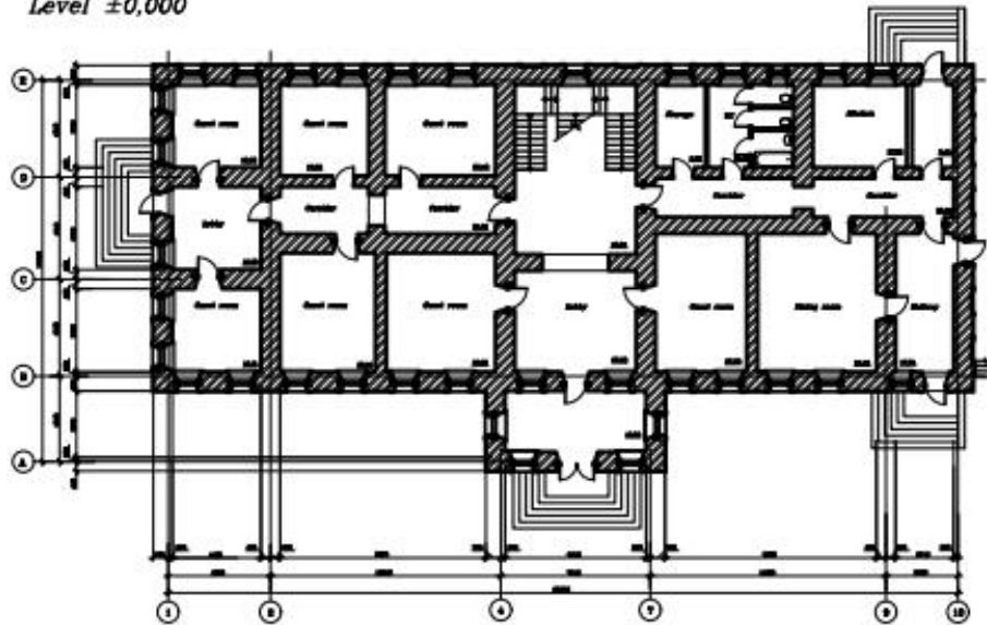
Level ±0,000
