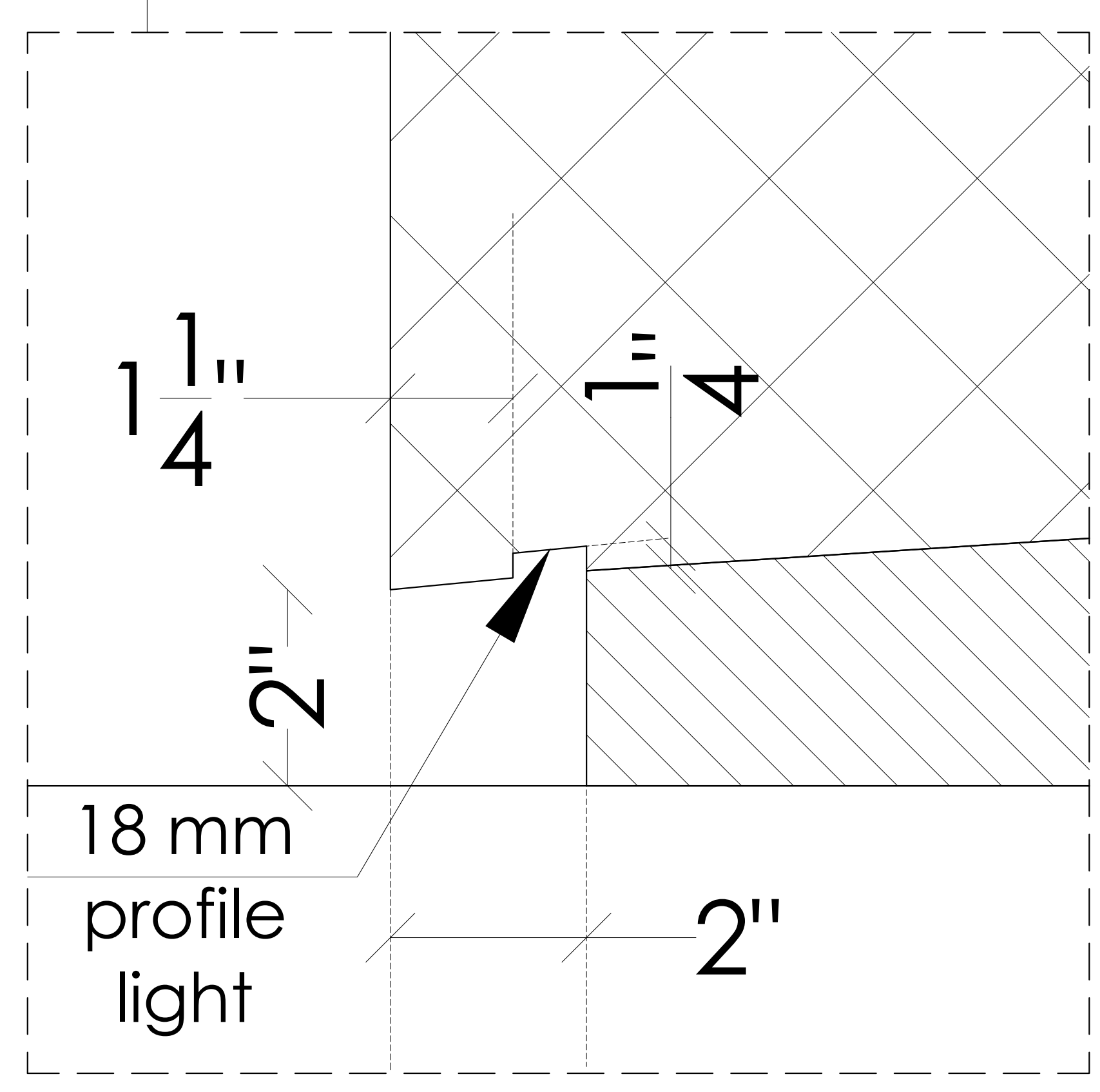
BED PROFILE LIGHT DETAIL
