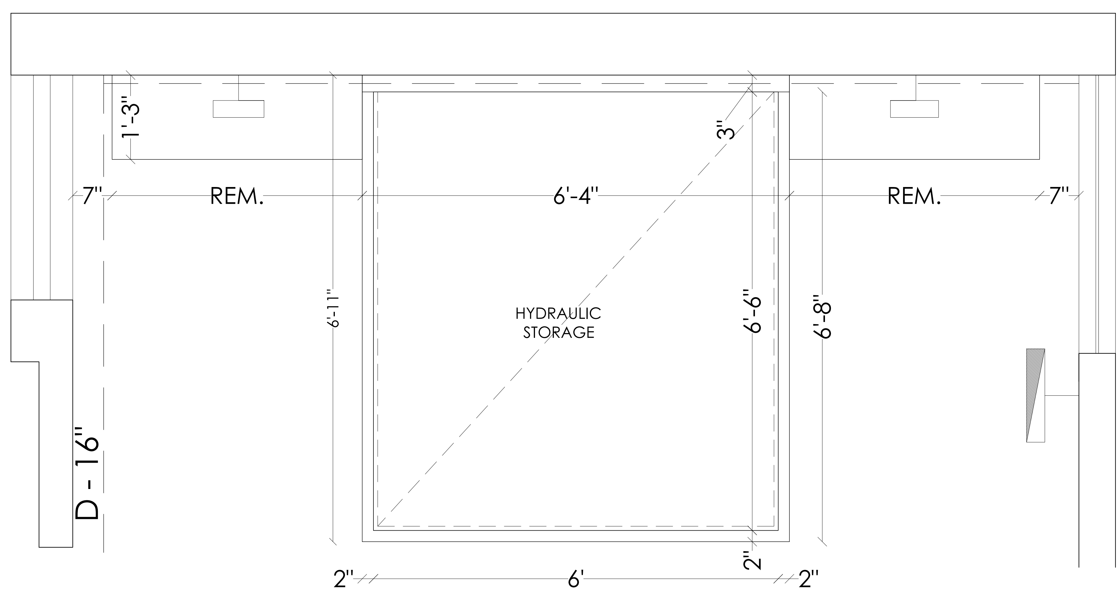
BED SIDE UNIT DETAIL
