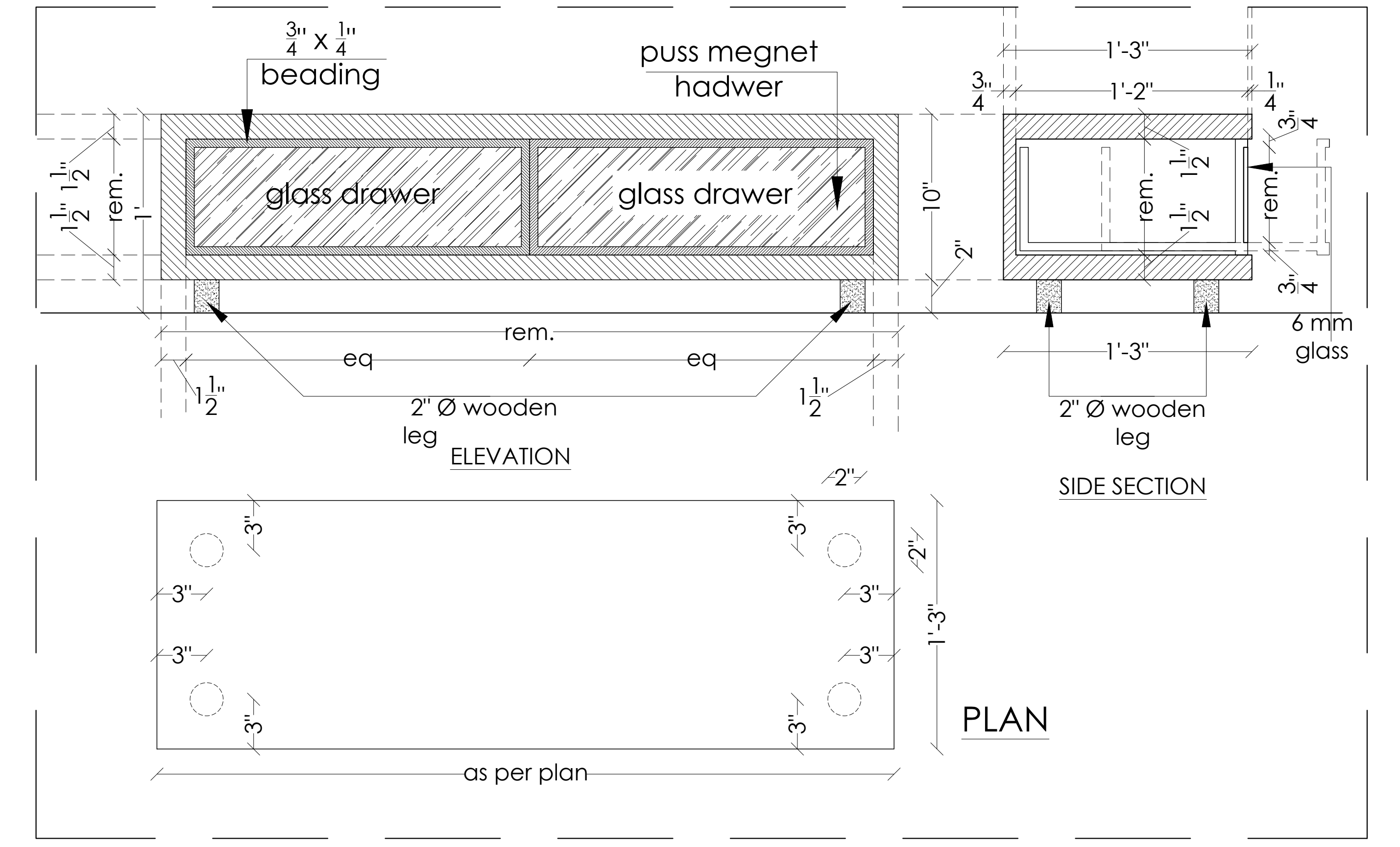
BED SIDE UNIT DETAIL
