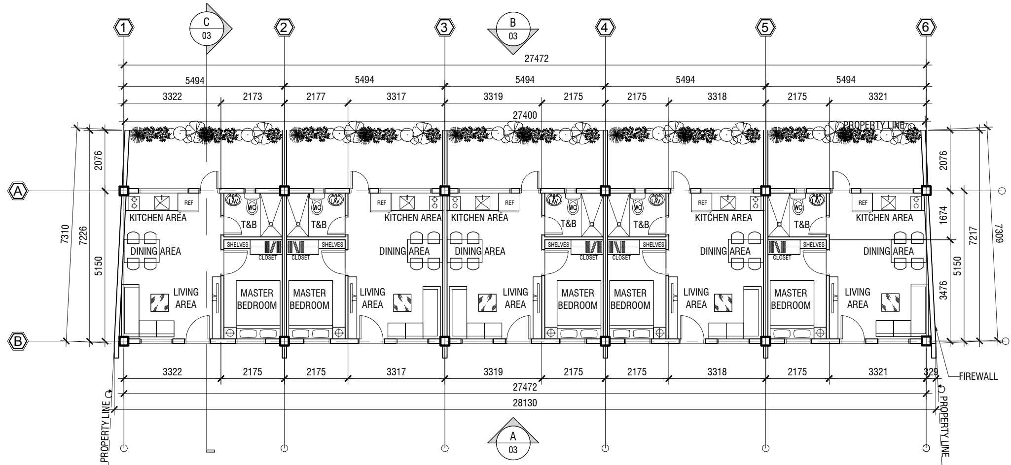
01 FLOOR PLAN PROPOSED APARTMENT LAYOUT 1:100 @ Ax
